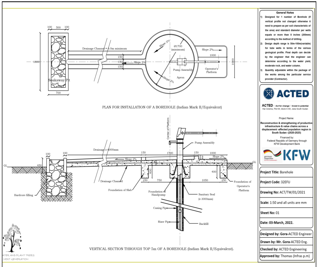
Figure 1: Plan and Sectional elevation of Borehole.
