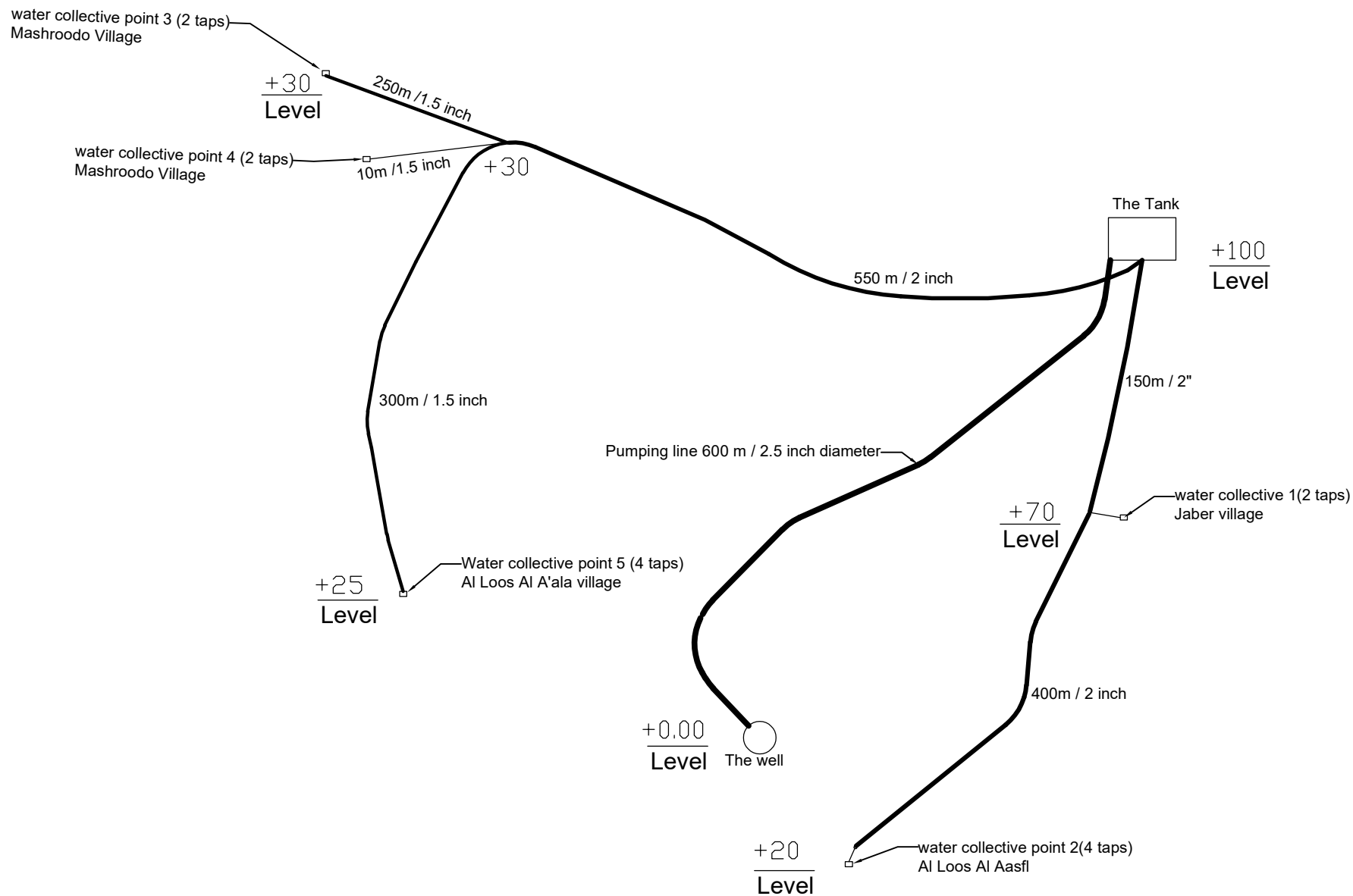
Plan of well, tank, and Water Collective points.
