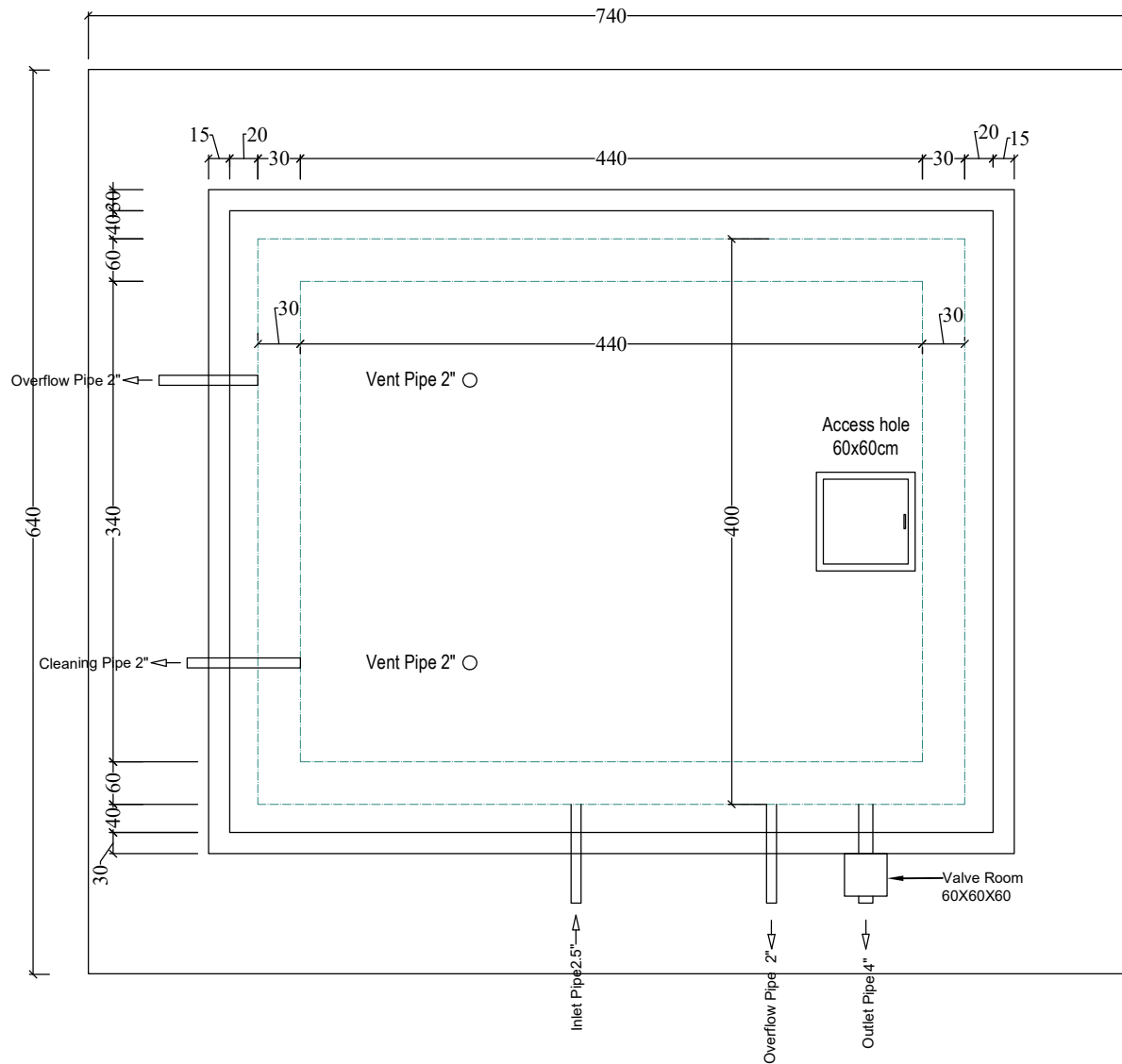
Plane of reinforced tank
