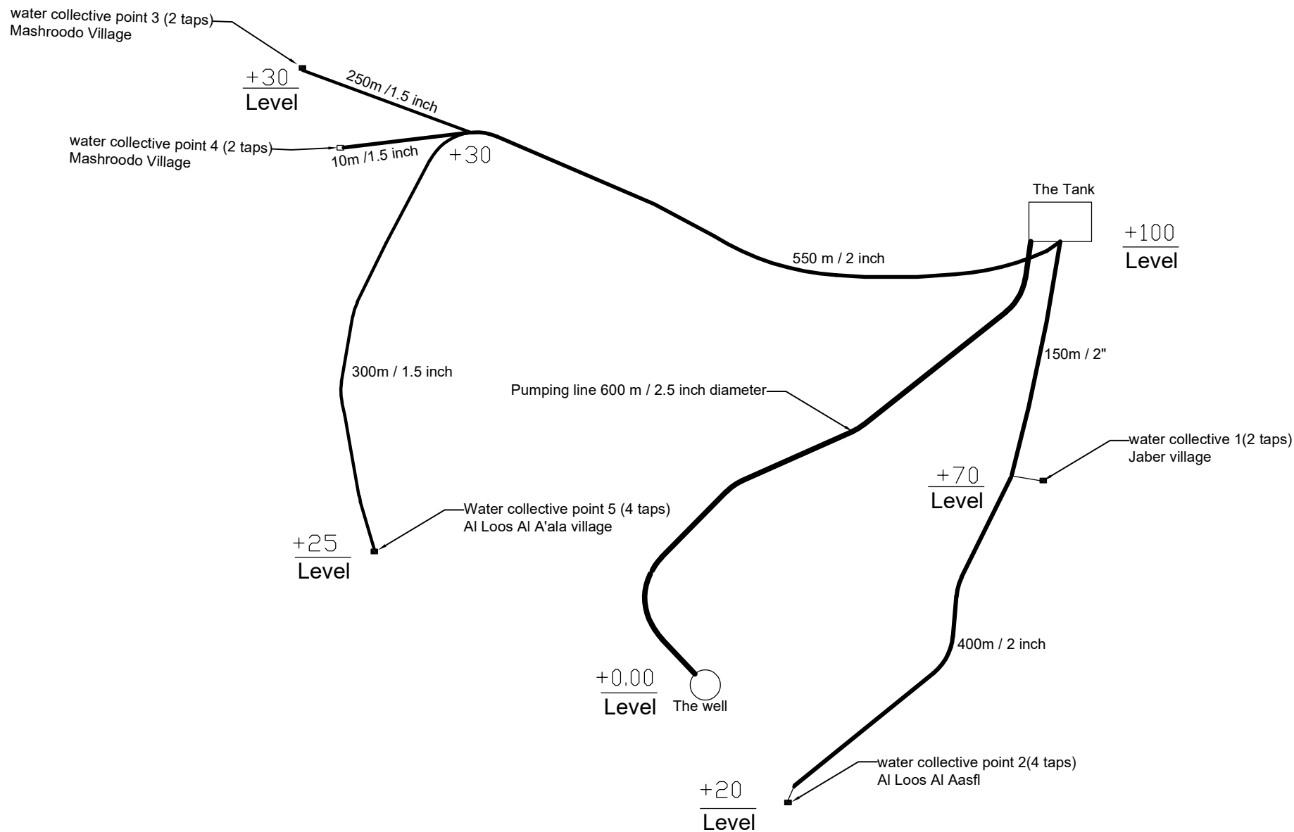
Plan of well, tank, and Water Collective points.
