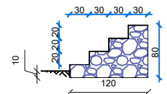
stair section
