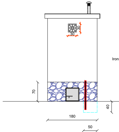
Latrine view
