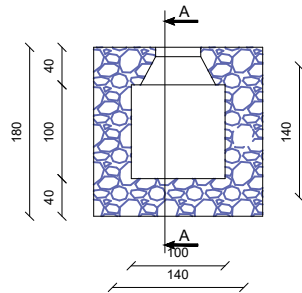
Foundation plan
