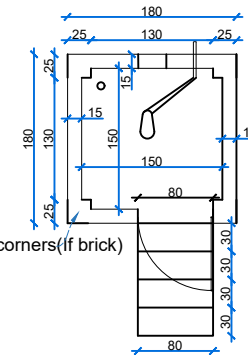
Floor plan
