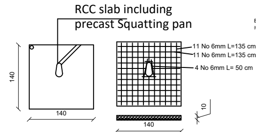
RCC Slab detail
